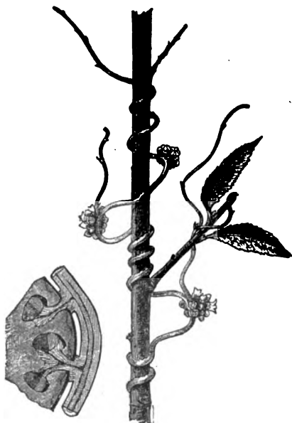
FIG. 59. — The Dodder, Cuscuta Europea ; \times \frac{1}{2} . It is here parasitic on Willow, on which it twines. Note the scale-like minute leaves, and the flowers in clusters. On the left is a section showing the connection of the haustorial roots with the veins of the host. (From Strasburger.)
